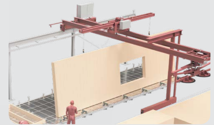
Turn-over and Transport Additional module to further reduce the load on the overhead crane
